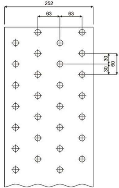
63x60-1/2" Fin-Lamel
